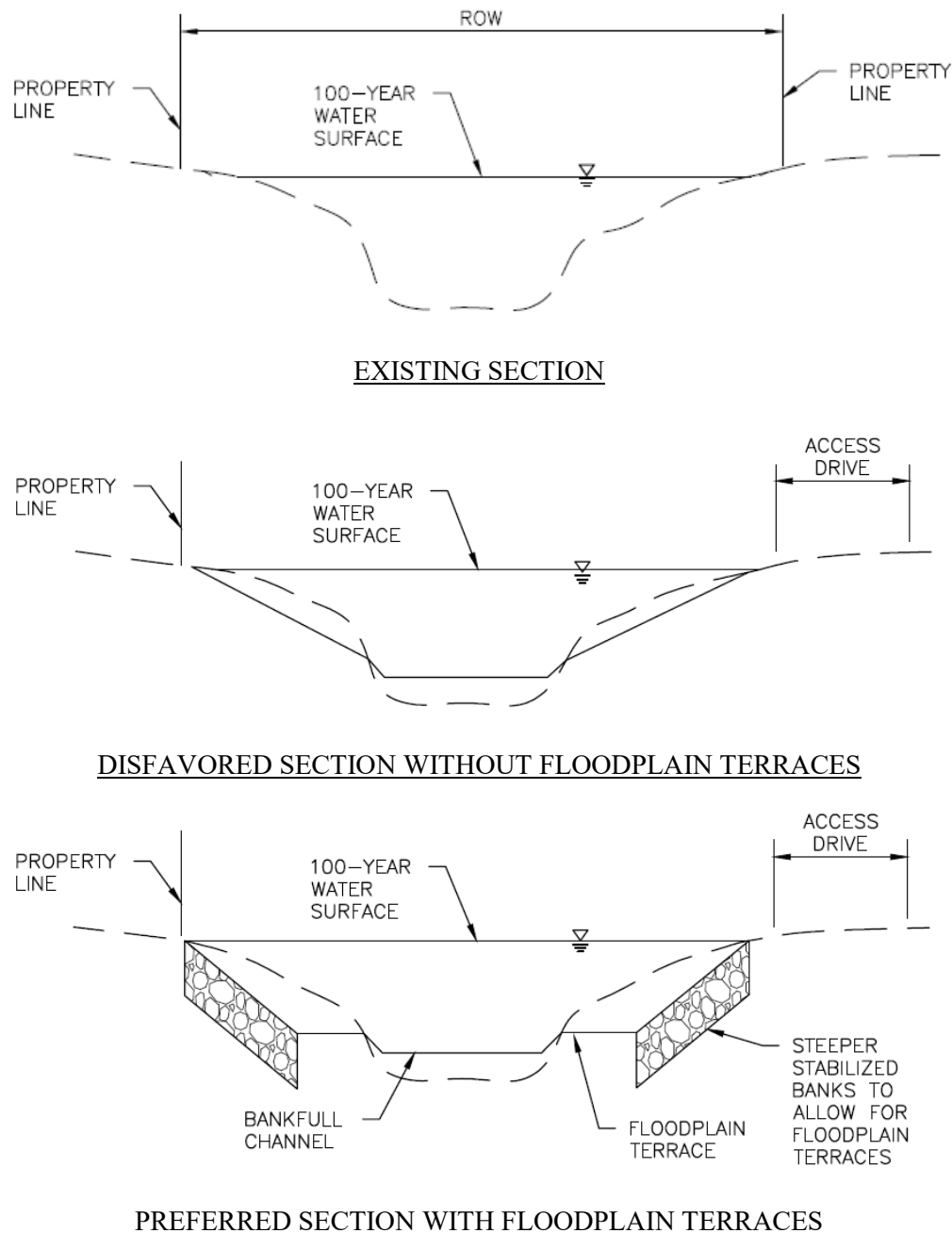
Figure 8-13. Creating floodplain terrace in narrow corridor
