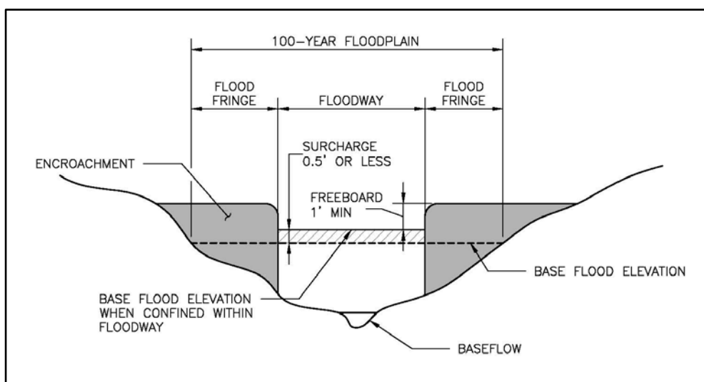
Figure 4-1. Floodway and flood fringe
