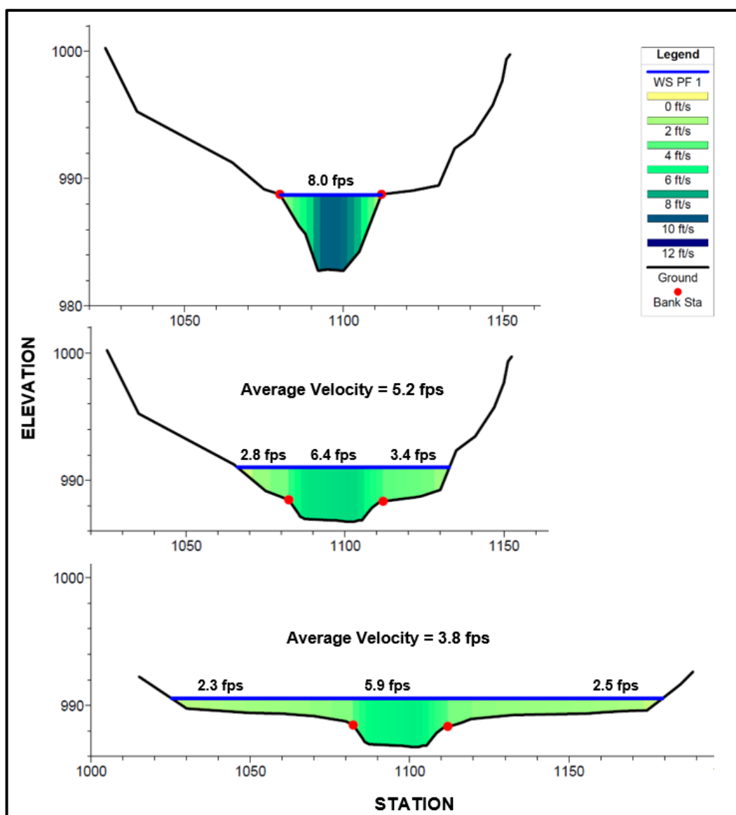
Figure 8-10. Impact of channel geometry on velocity
