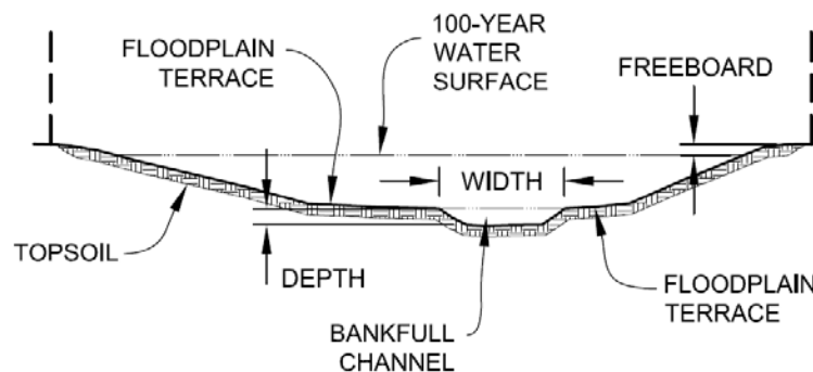
Figure 8-21. Typical naturalized channel geometry
